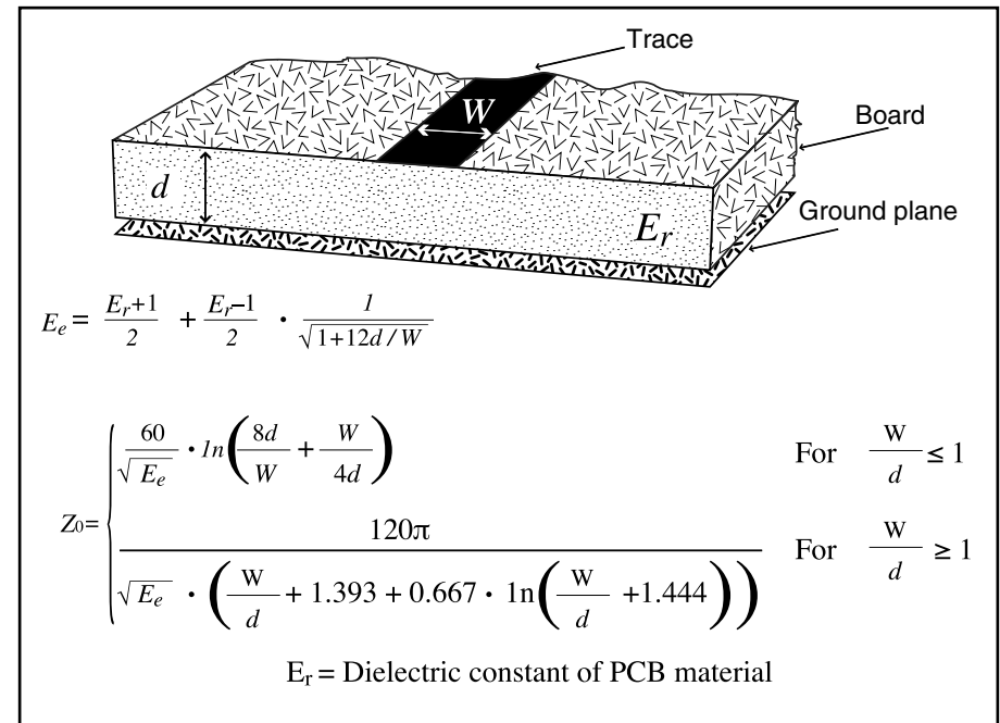
Figure 13: Microstrip Formulas
